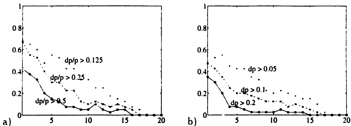
Figure 5-5: The fraction of posterior marginal estimates exceeding the specified error limits as a function of the number of positive findings that were treated exactly. The error measures used were a) the relative error, and b) the absolute error.
