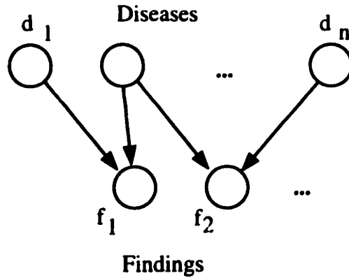
Figure 5-1: The QMR belief network is a two-level network where the dependencies between the diseases and their associated findings have been modeled via noisy-OR gates.
