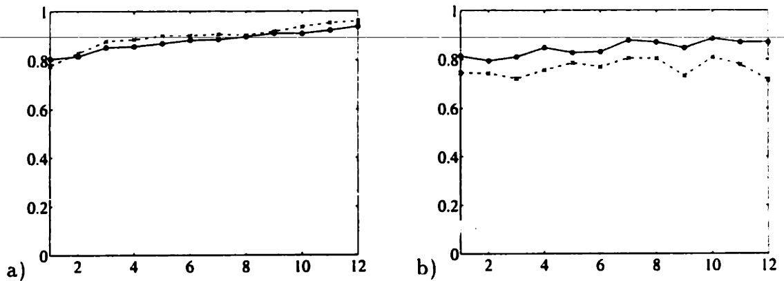
Figure 5-11: Mean correlation between the approximate posterior marginals and the min/max bounds as a function of the number of positive findings that were treated exactly. Solid line: correlation with the max-bound; dashed line: correlation with the min-bound. Figure a) is for the case where a proper ordering was used to select the findings to be treated exactly and in b) a random ordering was used.
