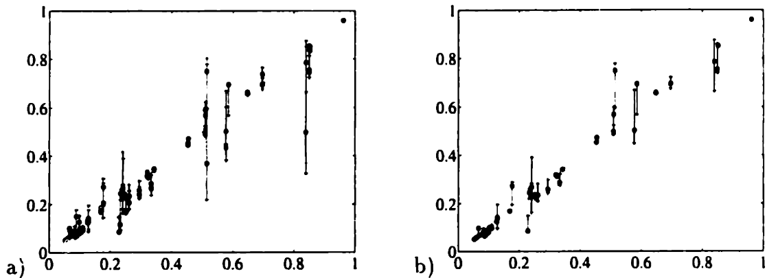
Figure 5-9: The correlation between the min/max bounds and the true posterior marginals. 10 most likely posterior marginals were included from each admissible case. In a) 8 findings were treated exactly and in b) 12.
