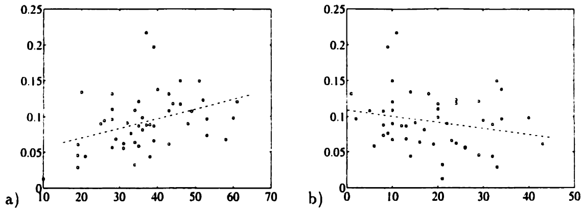
Figure 5-7: a) The variability \hat{\sigma} of the posterior marginals as a function of the number positive findings in the CPC-cases. b) The same variability measure \hat{\sigma} but now as a function of the number of negative findings. 8 positive findings were treated exactly for this figure.
