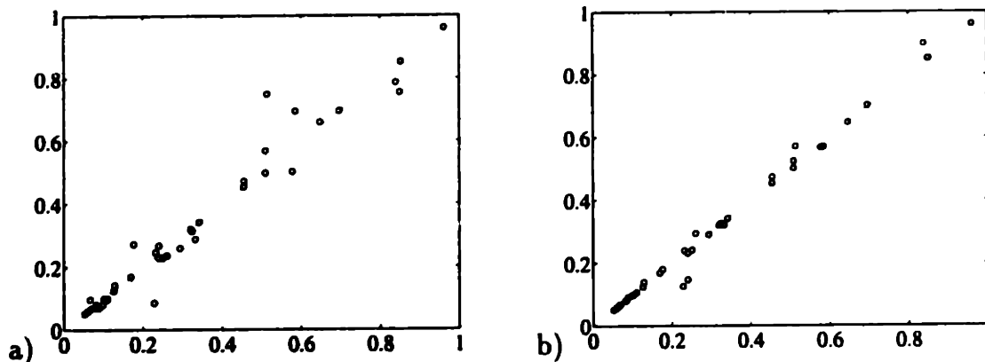
Figure 5-4: Correlation between the variational posterior estimates and the correct marginals. In a) 12 and in b) 16 positive findings were treated exactly.
