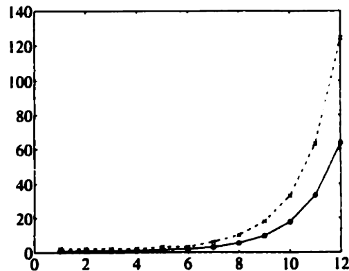
Figure 5-12: Mean (solid line) and maximum (dashed line) execution times in seconds for the analyses of section 5.6.2 across the CPC-cases as a function of the number of exactly treated positive findings.
