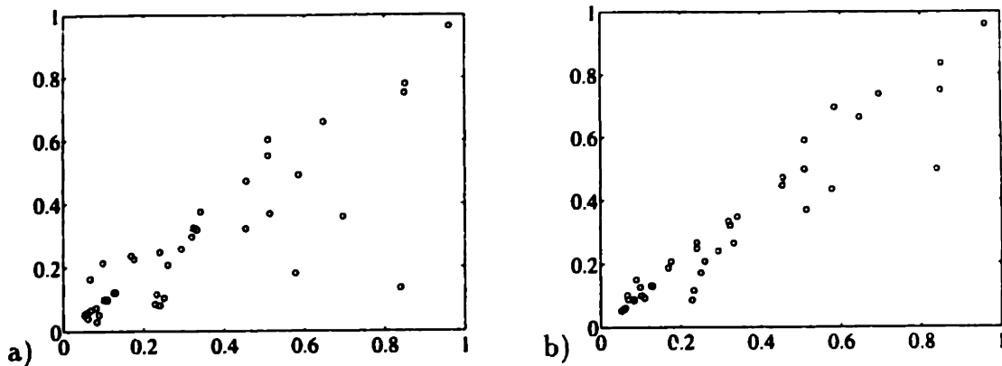
Figure 5-3: Correlation between the variational posterior estimates and the correct marginals. In a) 4 and in b) 8 positive findings were treated exactly.
