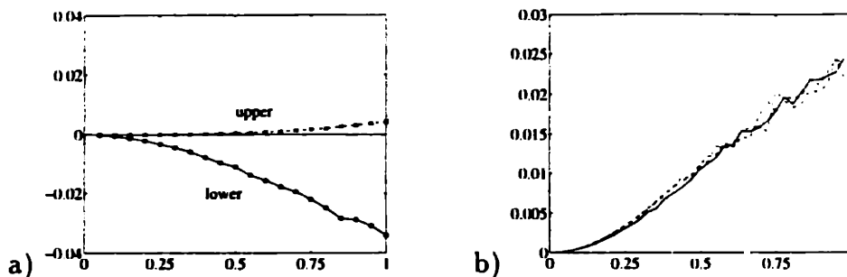
Figure 3-2: a) The mean relative errors in the log-partition function as a function of the scale of the random weights (uniform in [-d, d] ). Solid line: lower bound recursion; dashed line: upper bound. b) Mean relative difference between the upper and lower bound recursions as a function of d(n/8)^{1/2} , where n is the network size. Solid: n = 8 ; dashed: n = 64 ; dotdashed: n = 128 .
