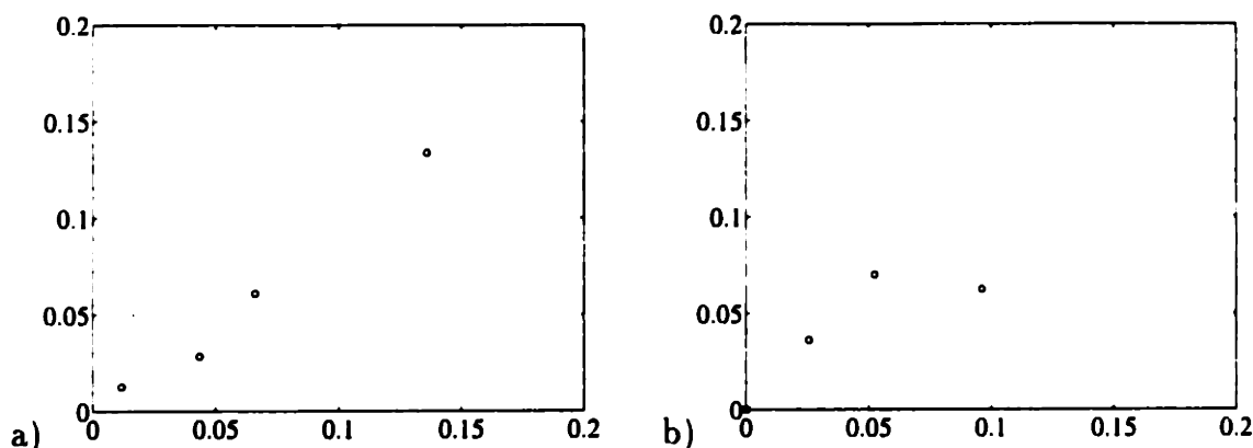
Figure 5-6: The correlation between \hat{\sigma} and \sigma , where \hat{\sigma} is the variability measure and \sigma is the true mean squared error between the variational estimates and the correct marginals. 10 most likely posterior marginals were included from each admissible case. The number of exactly treated findings was 8 in figure a) and 12 in b).
