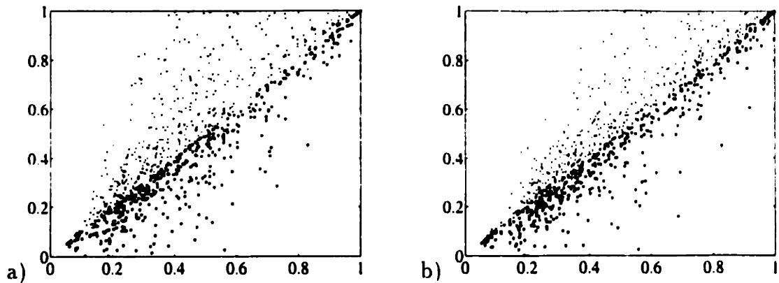
Figure 5-10: a) Correlation between the estimated posterior marginals and the min/max refined marginals. There were 8 positive findings considered exactly. b) as before but now the number of findings treated exactly was 12.
