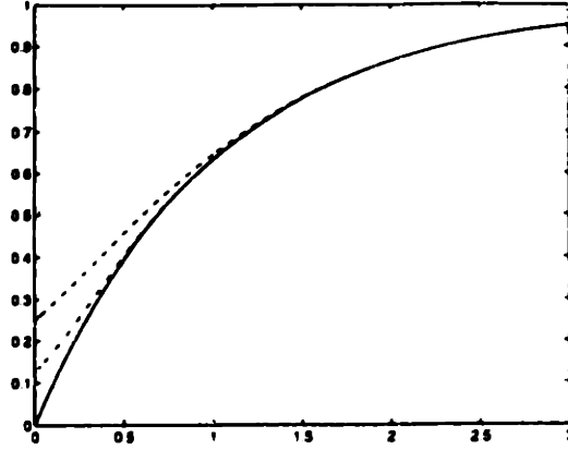
Figure 2-8: Accuracy of the noisy-OR expansion. Dotted line: N = 1 ; dashed line: N = 2 ; dot-dashed: N = 3 . N is the number of terms included in the expansion.
