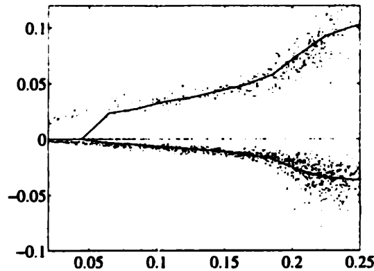
Figure 2-4: Noisy-OR network. Accuracy of the bounds for 8 by 8 two-level networks. The solid lines are the median relative errors in log-likelihood as a function of \sigma_{std} . The upper and lower curves correspond to the upper and lower bounds respectively.
